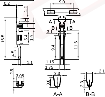
Male contact
