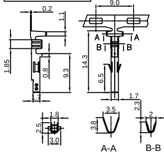
Female contact
