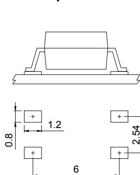
4-pin SOP
