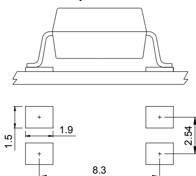
4-pin SMD
