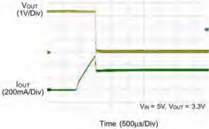
Output Current Limit Protection
