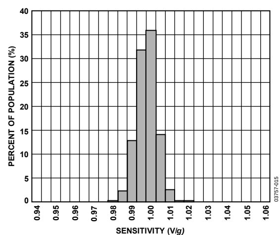
Figure 10. Y-Axis Sensitivity at 25°C
