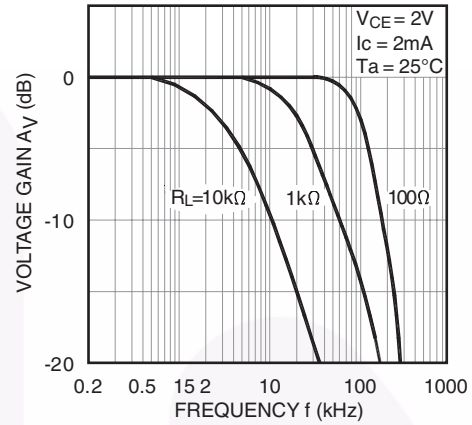
Fig. 14 Frequency Response
