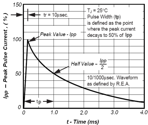
Fig3. Pulse Waveform
