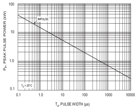
Fig5. Peak Pulse Power Rating curve
