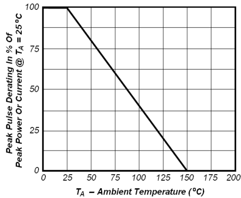
Fig1. Pulse Dearing Curve
