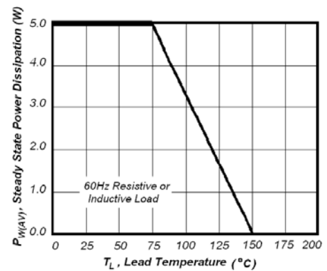
Fig6. Steady State Power Derating Curve
