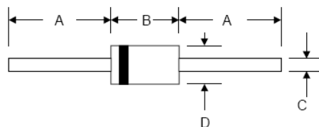
DO-15
