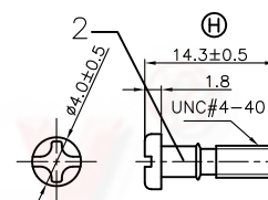
Short BOLT
