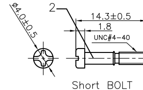
Short BOLT
