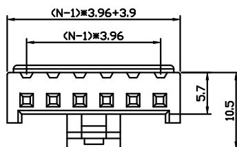
Femle Housing
