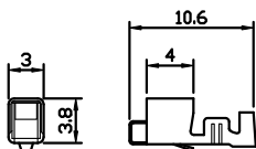
Femle Terminal
