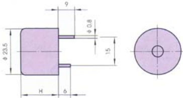
PIN(P) type
