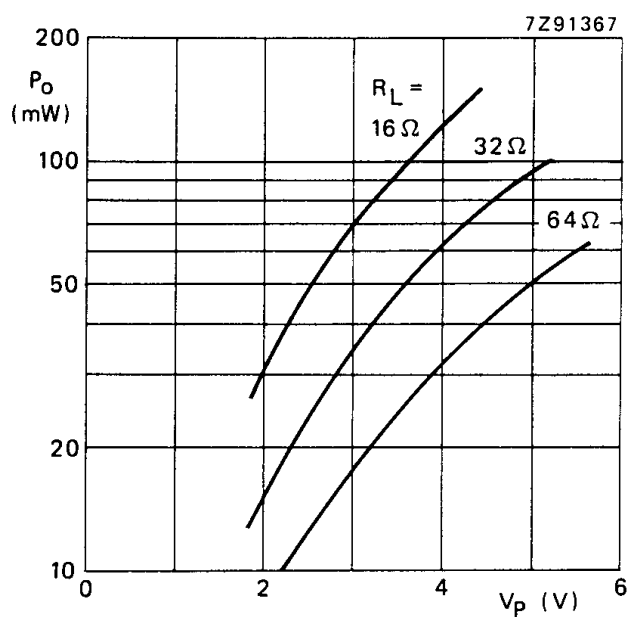
Fig.3 Output power across the load impedance ( R_L ) as a function of supply voltage ( V_p ) in stereo application. Measurements were made at f = 1\text{ kHz} ; d_{\text{tot}} = 10\% ; T_{\text{amb}} = 25\text{ }^\circ\text{C} .
