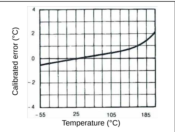
Figure 3. Calibrated error
