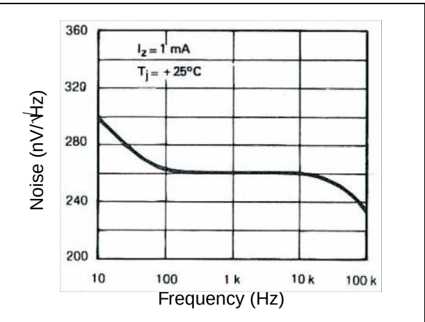
Figure 7. Noise voltage
