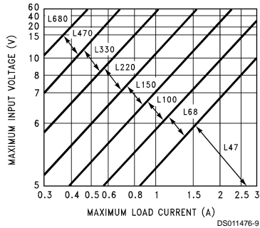
FIGURE 3. LM2576(HV)-3.3
