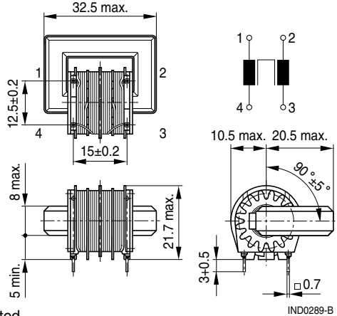
Horizontal version (B82734W)
