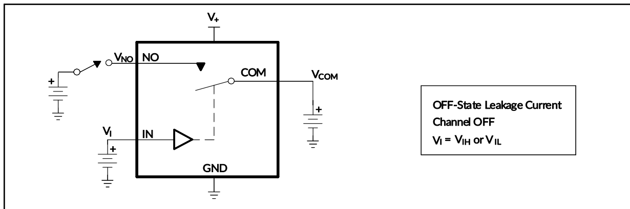
Figure 5. OFF-State Leakage Current ( I_{com(OFF)} , I_{No(OFF)} )
