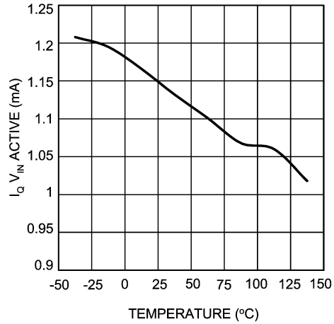
I Q Vin (Active) vs Temperature - "Y"
