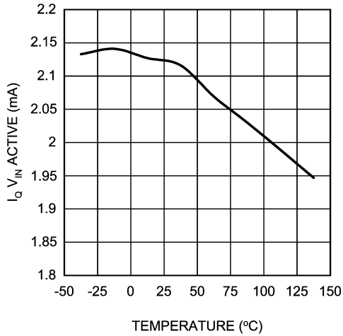
I Q Vin (Active) vs Temperature - "X"
