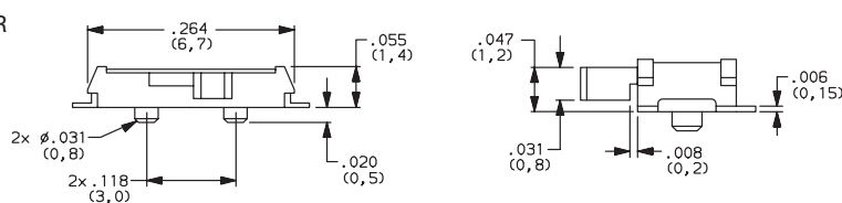
PCM12SMTR SPDT
