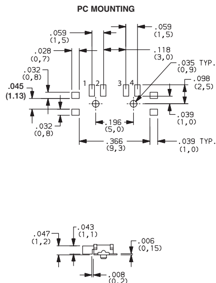
PCM13SMTR SP3T
