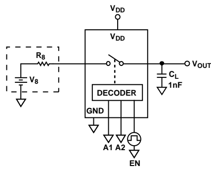
Figure 24. Charge Injection
