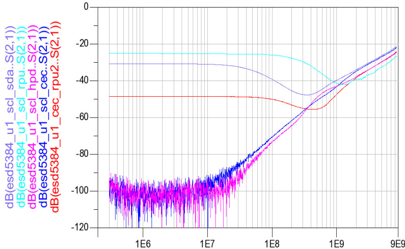
Figure 2. Crosstalk Measurements
