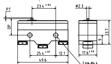
Z-15G-B
