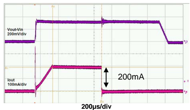
Reverse-Current Limit
