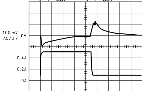
Load Transient Response for Continuous Mode V_{IN} = 20V , V_{OUT} = 5V , L = 100\ \mu\text{H} , C_{OUT} = 100\ \mu\text{F} , C_{OUT}ESR = 0.1\ \Omega
