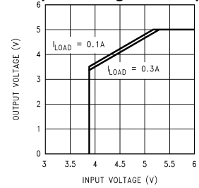
Dropout Voltage—5.0V Option
