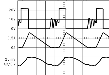
Discontinuous Mode Switching Waveforms V_{IN} = 20V , V_{OUT} = 5V , I_{LOAD} = 300\text{ mA} L = 15\ \mu\text{H} , C_{OUT} = 68\ \mu\text{F} (2x), C_{OUT}ESR = 25\ \text{m}\Omega
