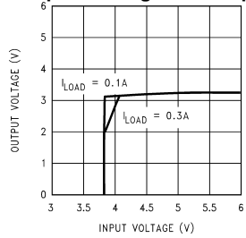
Dropout Voltage—3.3V Option
