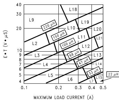
Figure 12. LM2674-ADJ
