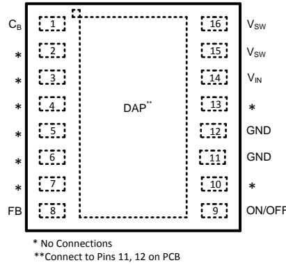
Figure 1. 16-Lead LLP Surface Mount Package Top View
