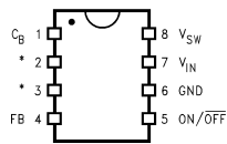
Figure 2. SO-8/DIP Package 8-Lead Package Top View
