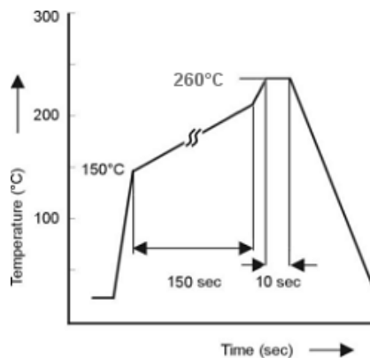
soldering condition
