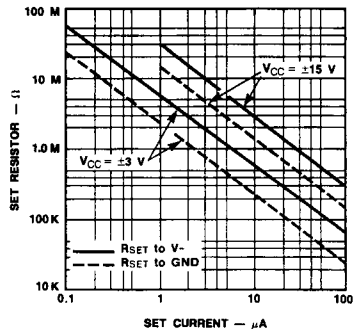
Set Current vs Set Resistor
