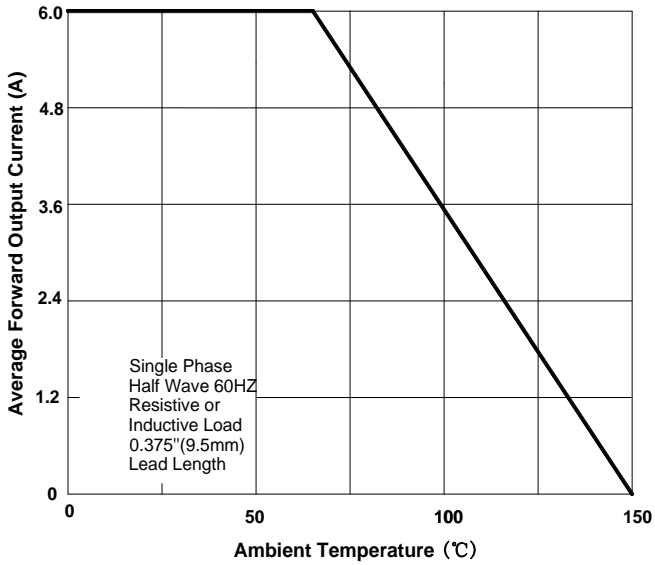
FIG.1: Io-Ta Curve
