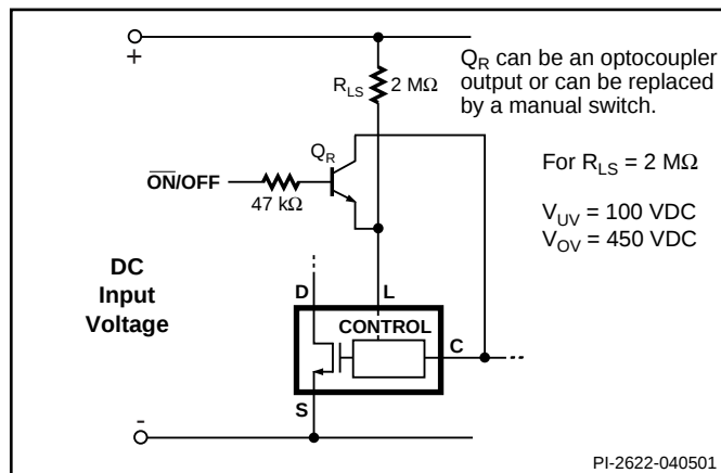
Figure 26. Active-off Remote ON/OFF with LINE-SENSE.
