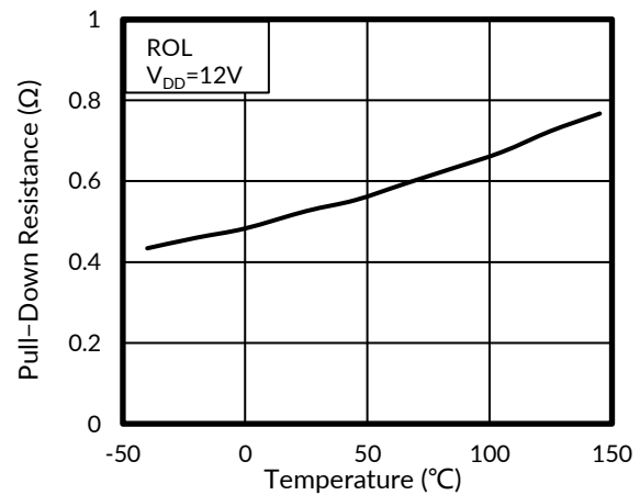
Figure 12. Output Pulldown Resistance vs Temperature
