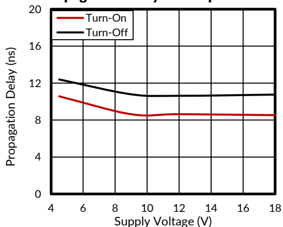
Figure 17. Non-Inverting Propagation Delays vs Supply Voltage
