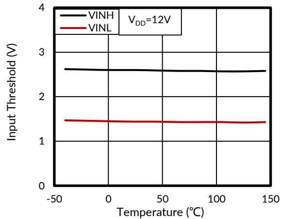
Figure 10. Input Threshold vs Temperature
