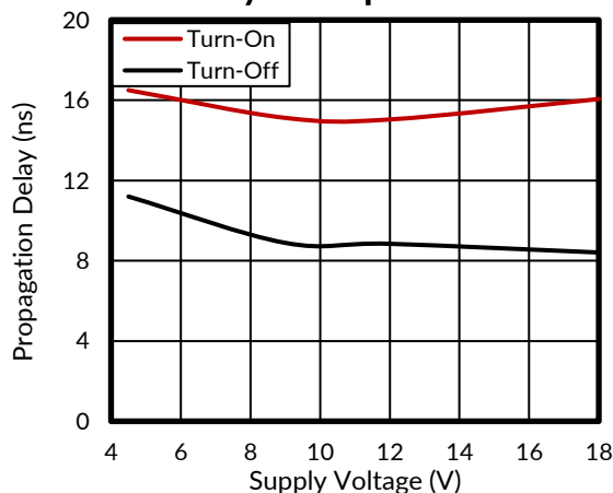
Figure 18. Inverting Propagation Delays vs Supply Voltage
