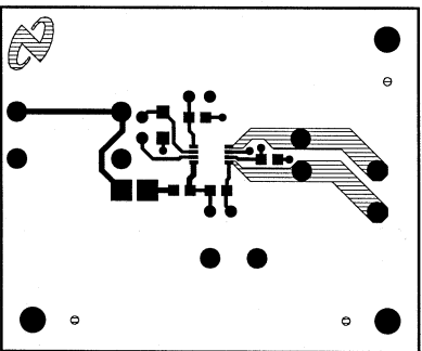
Figure 76. Top Layer
