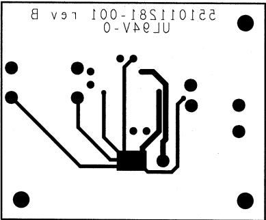
Figure 74. Bottom Layer
