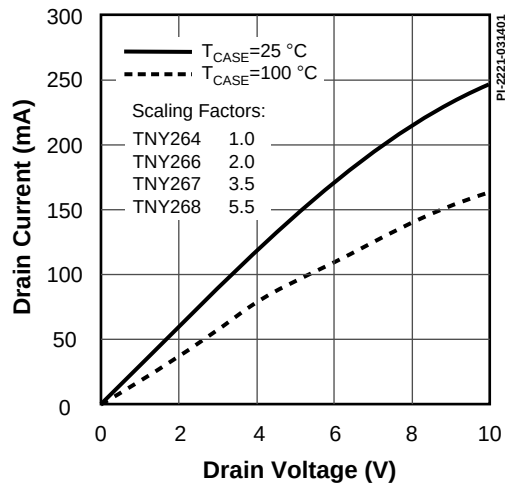
Figure 27. Output Characteristic.
