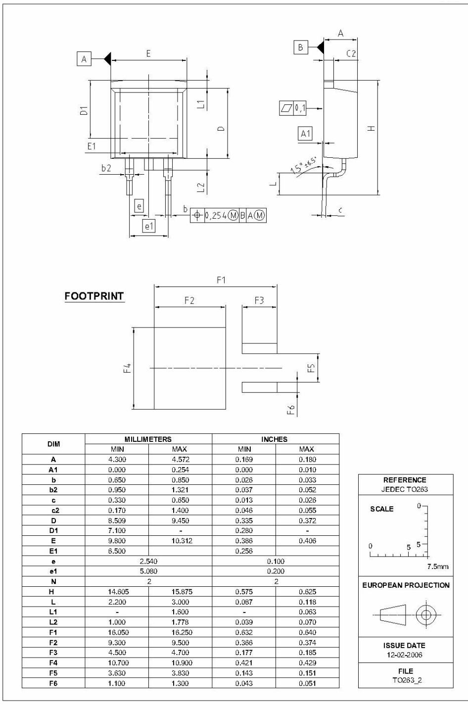
PG-TO263-3-2
