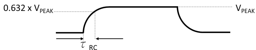
Fig.16 Waveforms of dV/dt
