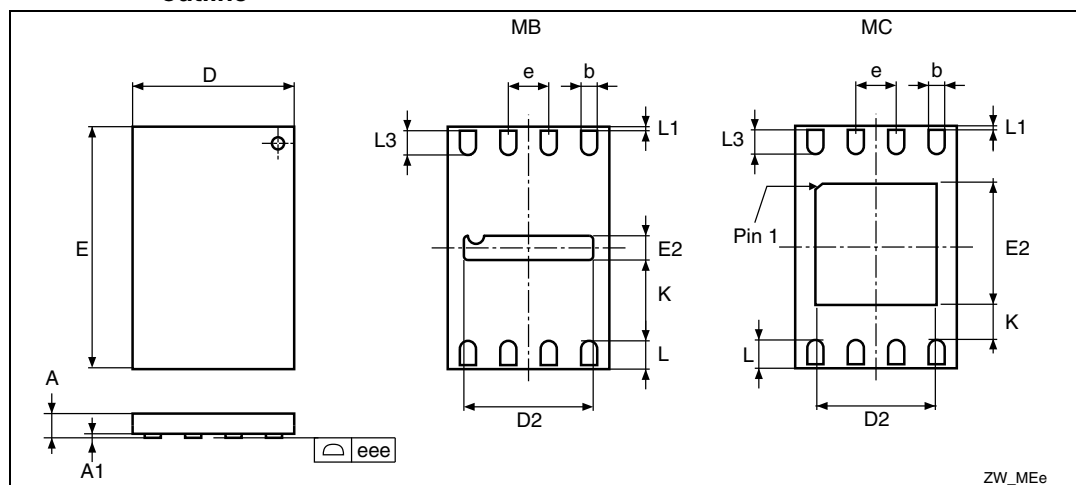
Figure 19. UDFPN8 (MLP8) - 8-lead ultra thin fine pitch dual flat no lead, package outline
