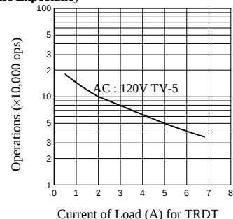
Life Expectancy
