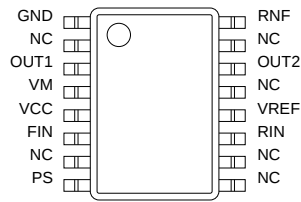
Fig.30 BA6285FS (SSOP-A16)
