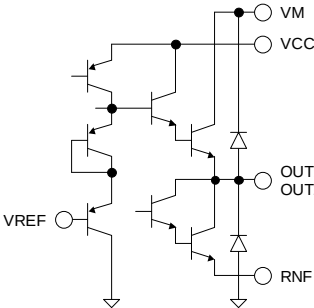
(BA6285FS, BA6285AFP-Y, BA6920FP-Y) Fig.39 POWER SAVE
