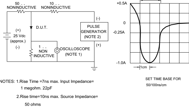
FIG.4-TEST CIRCUIT DIAGRAM AND REVERSE RECOVERY TIME CHARACTERISTIC
