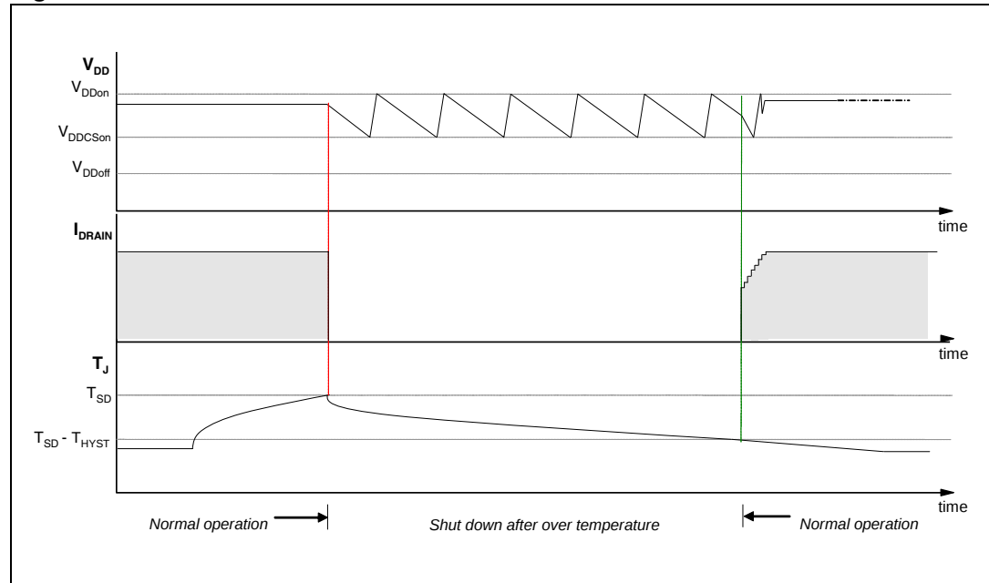
Figure 16. Thermal shutdown
