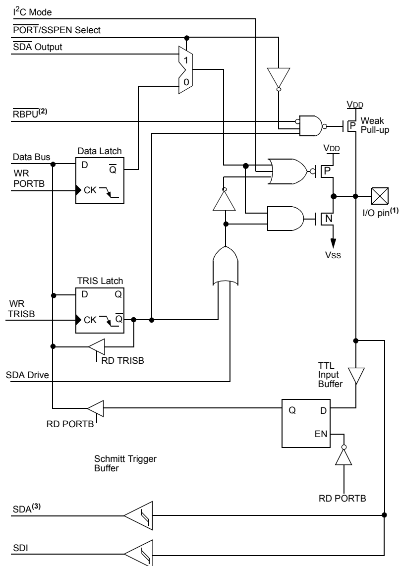
FIGURE 5-9: BLOCK DIAGRAM OF RB1 PIN
