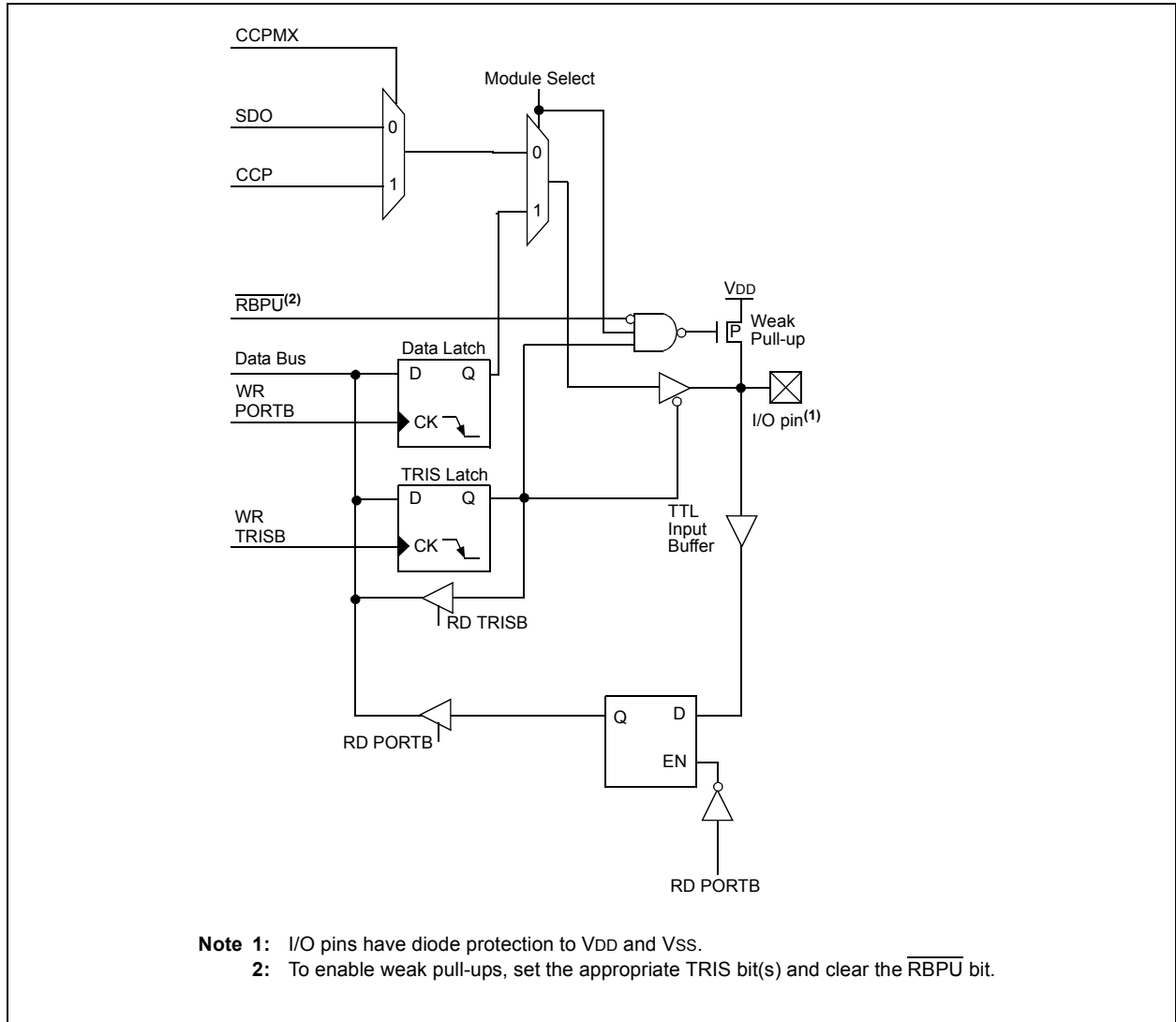
FIGURE 5-10: BLOCK DIAGRAM OF RB2 PIN
