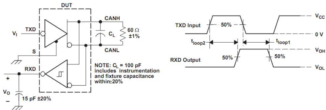
Figure 9. t(LOOP) Test Circuit and Waveforms
