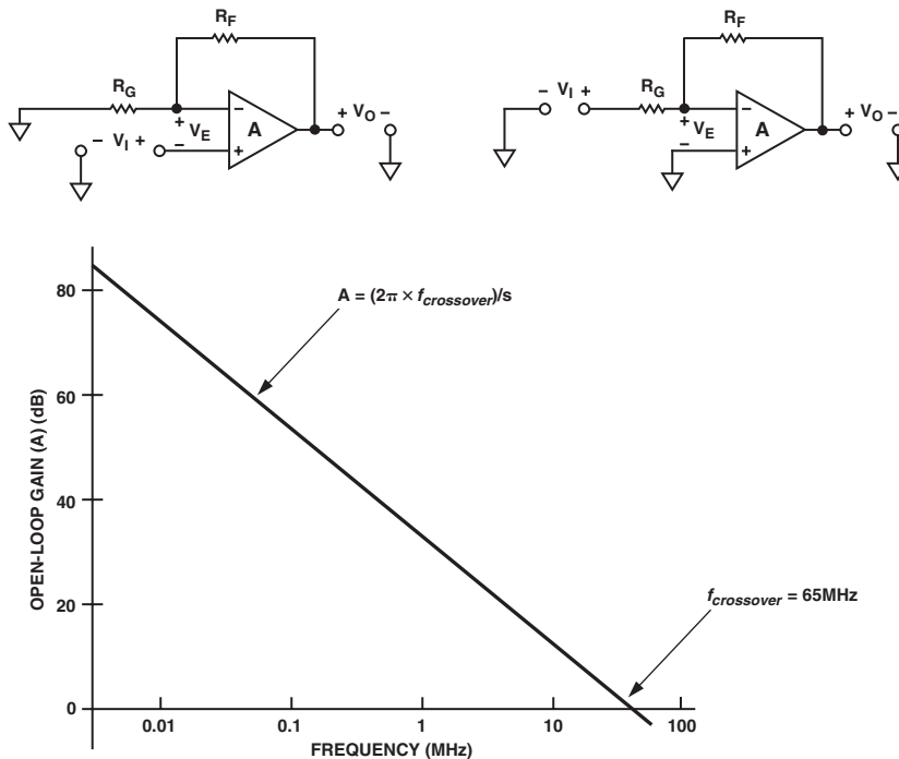
Figure 3. Open-Loop Gain vs. Frequency and Basic Connections
