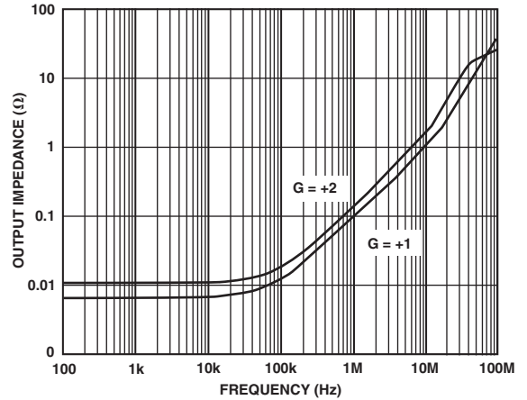
TPC 34. Output Impedance vs. Frequency (See Test Circuits 4 and 6)
