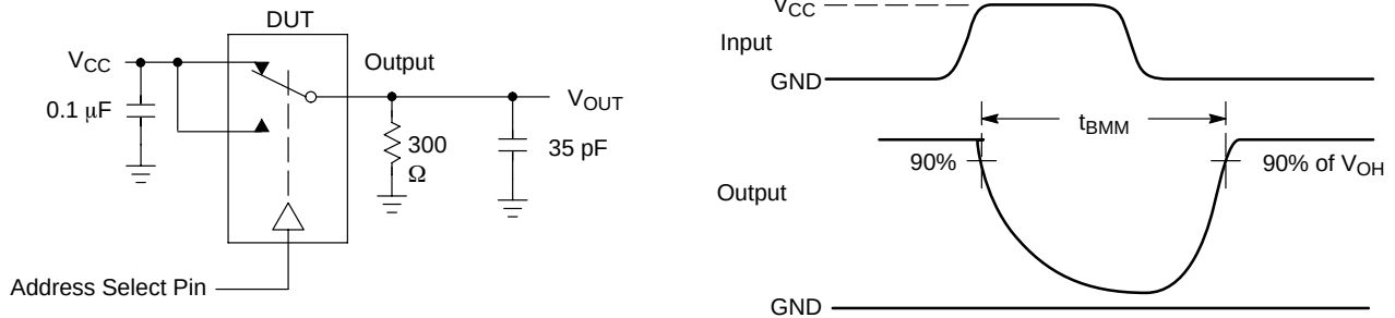
Figure 19. t_{BMM} (Time Break-Before-Make)
