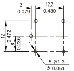
Mounting (Bottom view)
