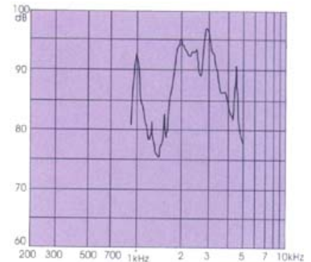
TFM-27DT 9V P-P Square Wave/10cm
