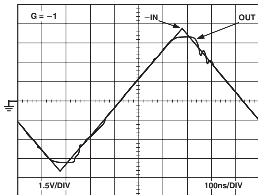
TPC 21. Output Overdrive Recovery (See Test Circuit 3), V_S = \pm 5 V
