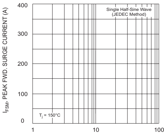
NUMBER OF CYCLES AT 60 Hz Fig. 3 Max Non-Repetitive Surge Current
