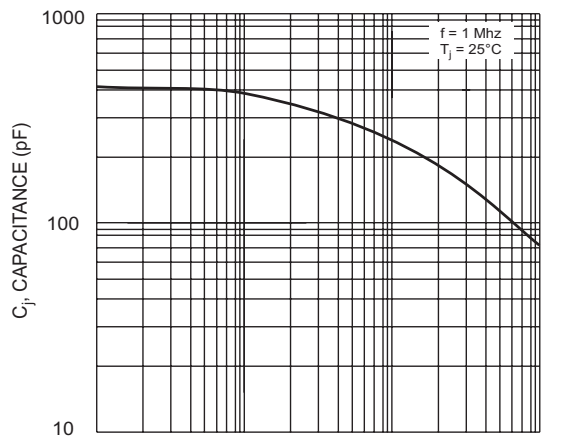
V_R , REVERSE VOLTAGE (V) Fig. 4 Typical Junction Capacitance (per element)
