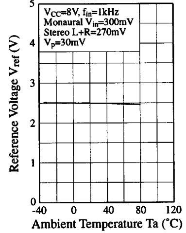
V_{REF} - T_a
