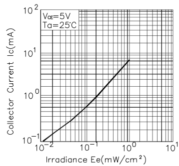
Fig.3 Collector Current vs. Irradiance
