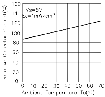
Fig.2 Relative Collector Current vs. Ambient Temperature
