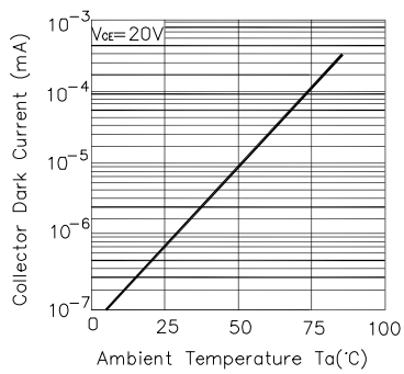
Fig.4 Collector Dark Current vs. Ambient Temperature
