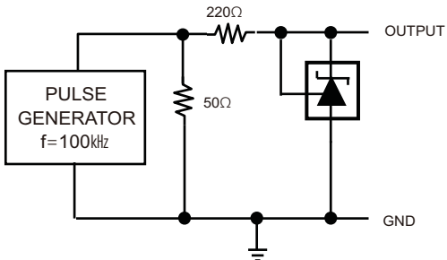
FIGURE 4. TEST CIRCUIT FOR PULSE RESPONSE
