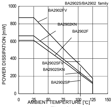
Fig. 73 Derating Curve
