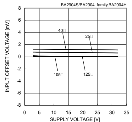
Fig. 60 Input Offset Voltage - Supply Voltage (VICM=0[V], VOUT=1.4[V])
