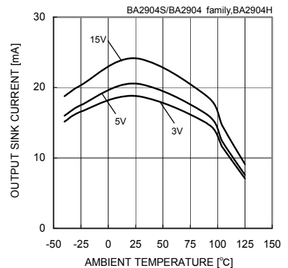
Fig. 57 Output Sink Current - Ambient Temperature (VOUT=VCC)
