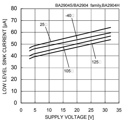
Fig. 58 Low Level Sink Current - Supply Voltage (VOUT=0.2[V])
