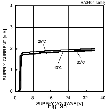
Fig. 98 Supply Current - Supply Voltage
