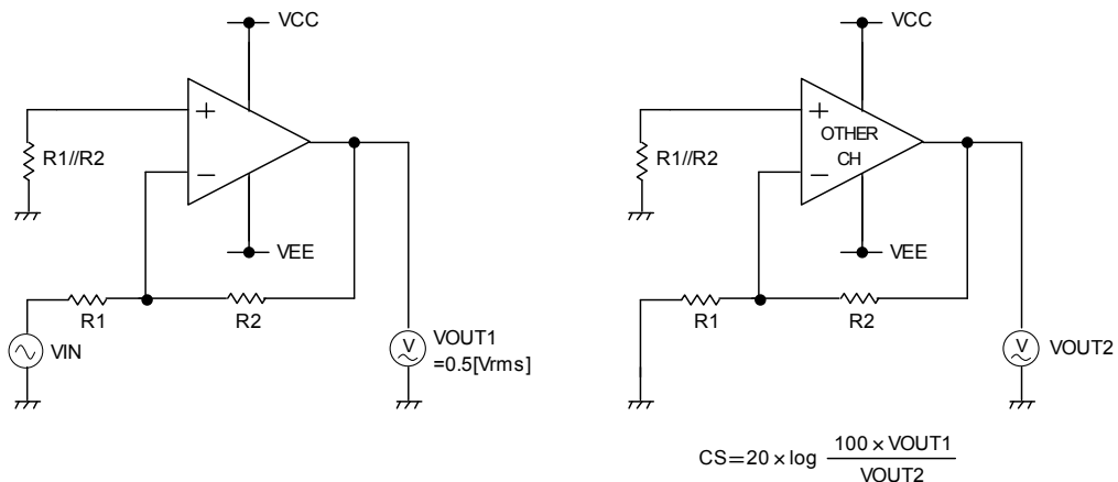
Fig. 123 Measurement Circuit 3
